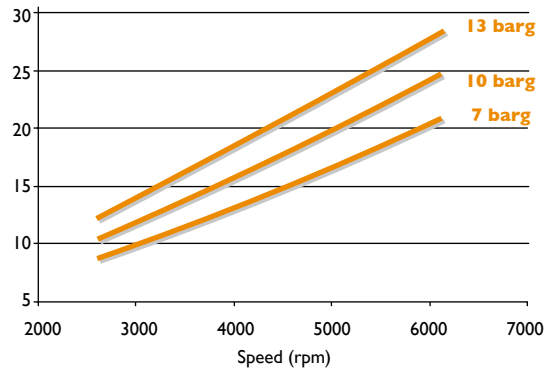
Power (HP)
